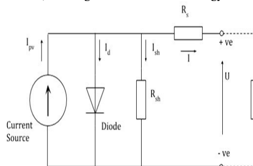
Fig 2. Equivalent Circuit of PV Module
