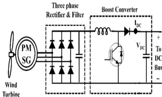
Fig 4. Equivalent Circuit of Wind energy System
