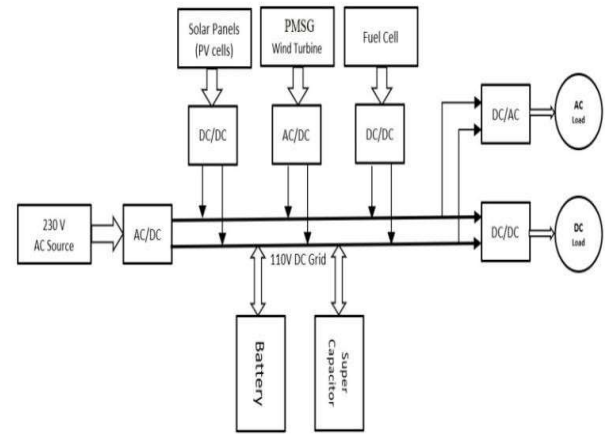
Fig 1. Configuration of DC Microgrid
