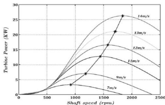
Fig 5. Characteristics Curve of wind Module
